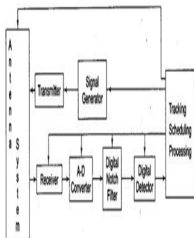
Fig. 15.45 Block Diagram of a Modern Radar System
